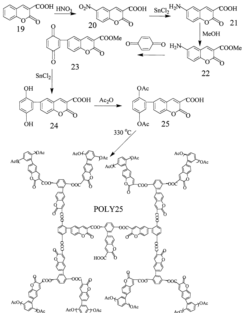
Scheme 5 Synthesis of coumarin containing hyperbranched polymer
