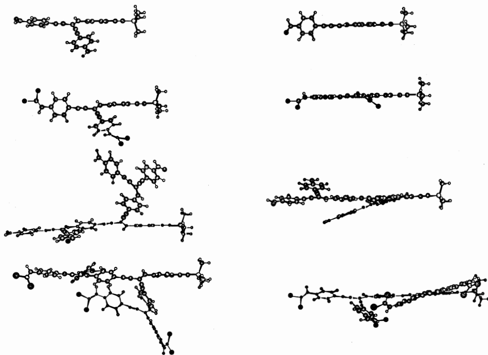
Fig. 3. PM3 optimized geometries of some conjugated dendrimers
