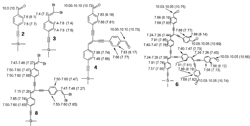
Fig. 2 Experimentally observed and theoretically calculated chemical shifts of some dendrimers.
