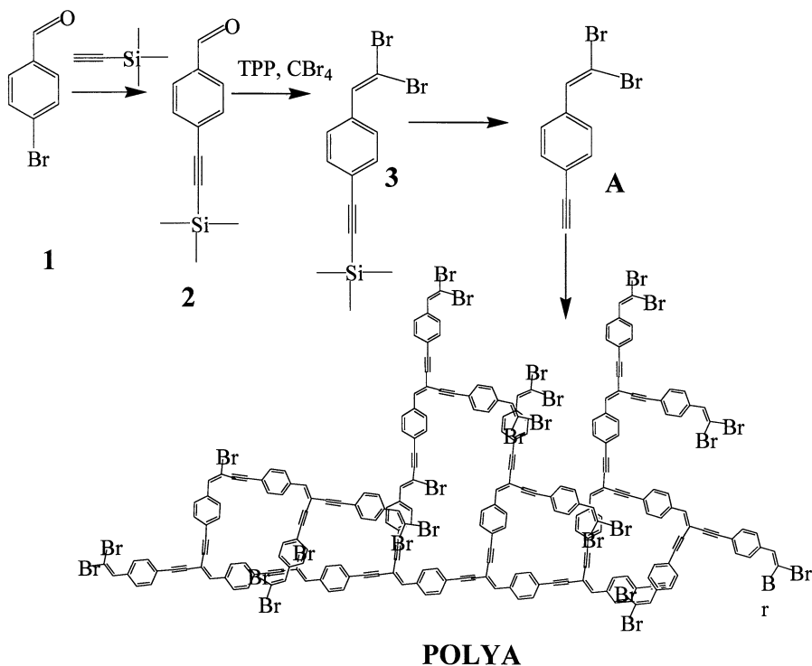
Scheme 1 Synthetic route to POLYA
