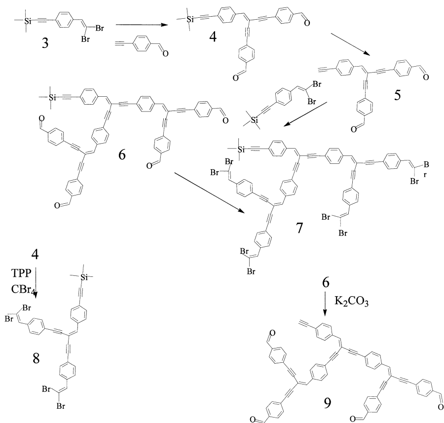
Scheme 2 Synthetic route well defined hyperbranched oligomers
