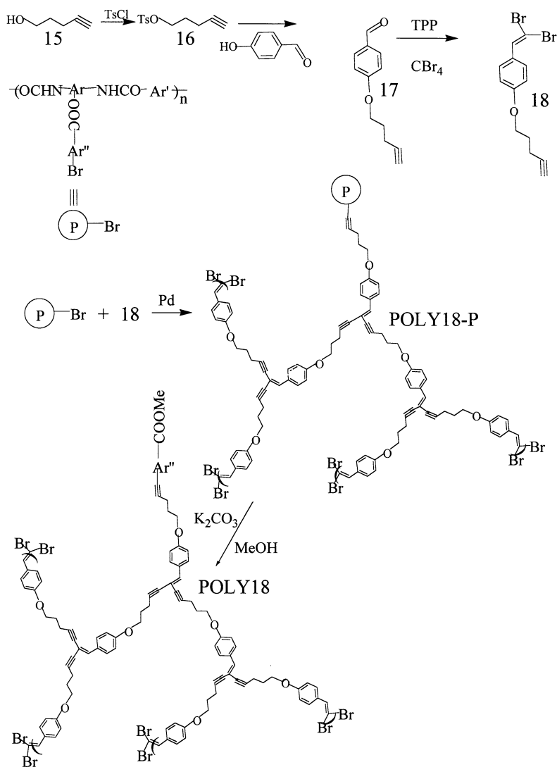
Scheme 4 Polymer supported hyperbranched polymer synthesis
